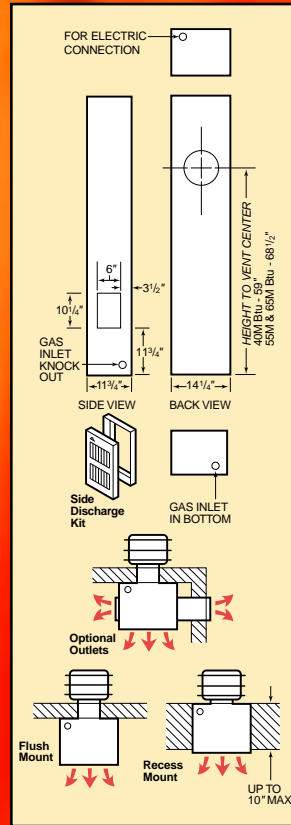
Standard Vent Assembly — Direct Vent Counterflow — accommodates wall thickness from 3/4" (recessed) to 12" (packaged separately).
