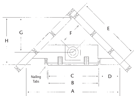
Unit and Framing Specifications (inches)
