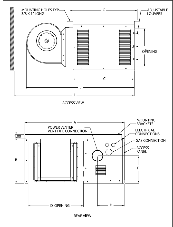
Figure 18.2 - Dimensional Drawings - Model HDB
