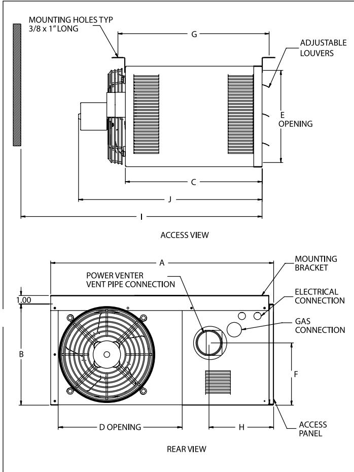
Figure 18.1 - Dimensional Drawings - Model HD
