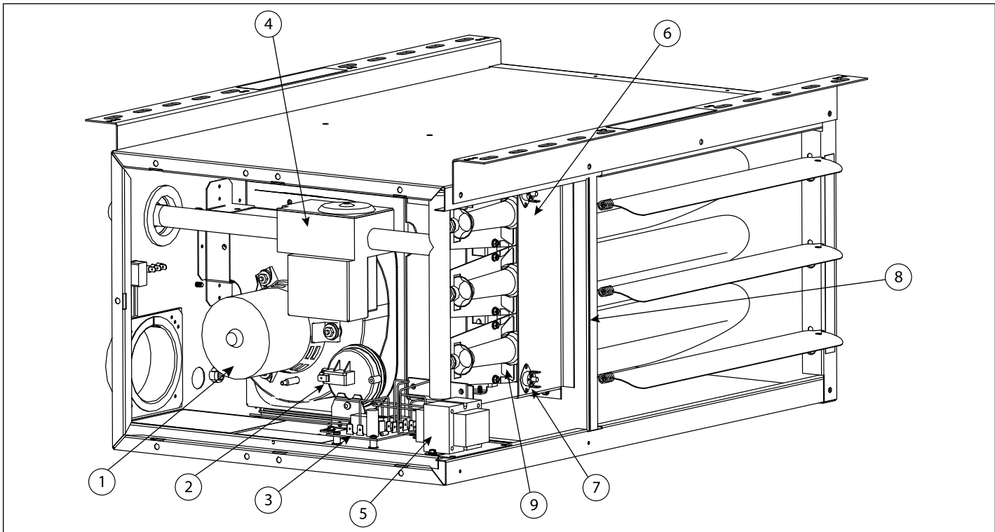
Figure 4.1 - Factory Mounted Standard and Optional Features (Models HD/HDB)
