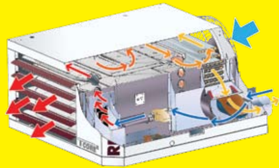
TCore 3 ™ Heat Exchanger (patent pending)
