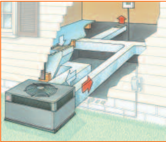
Packaged Air Conditioner System
